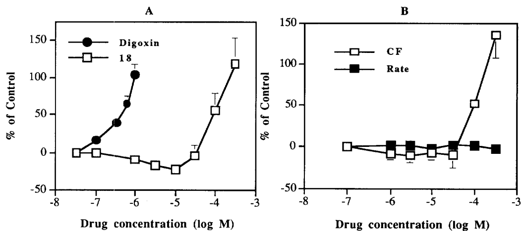
Figure 2. Panel A: Effect of digoxin and compound 18 on the peak contractile force in isolated guinea-pig electrically driven left atria. Panel B: Effect of compound 18 on the rate (Rate) and peak contractile force (CF) of spontaneous contractions in isolated guinea-pig right atria. Ordinate: % of control values. Abscissa: drug concentration (log M). Each point represents the mean of at least five experiments; vertical bars represent the S.E.M.
